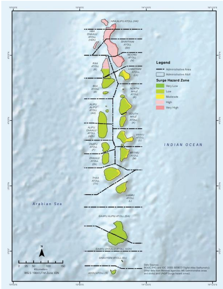
Figure 17: Maldives surge hazard zone (source; CLIMATE RISK COUNTRY PROFILE: MALDIVES)
