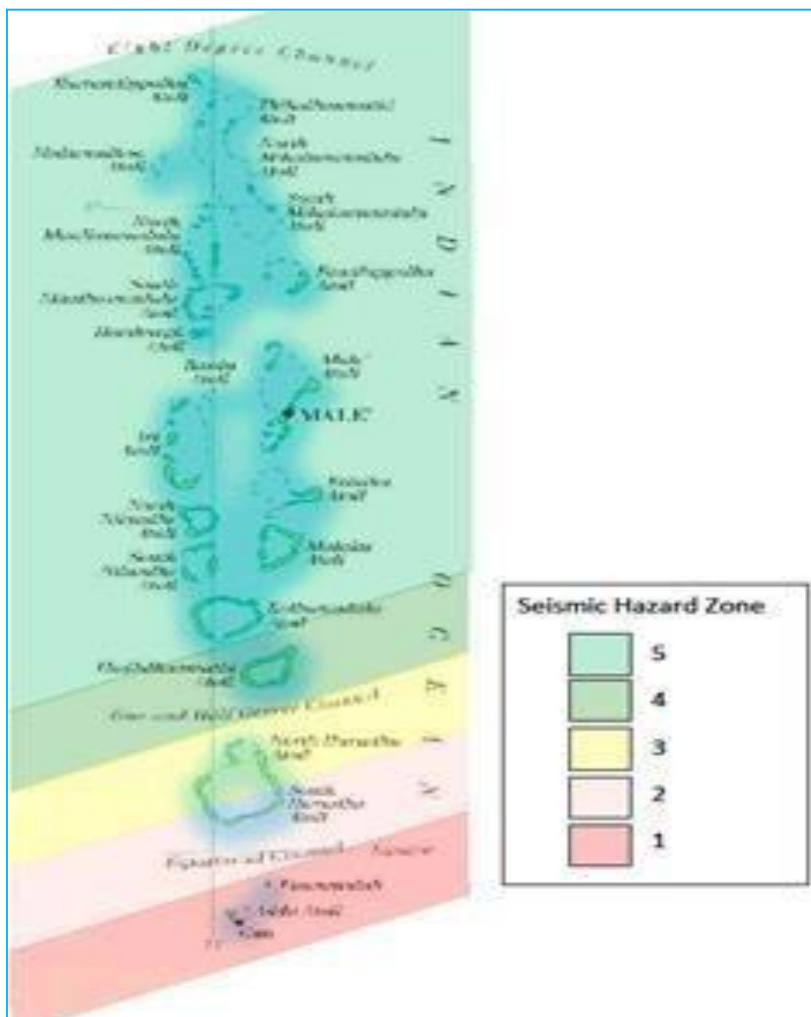
Figure 18: Earthquake seismic hazard zones
