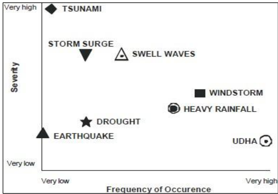
Figure 13: Hazards and Patterns in Maldives, Diagram 2007
