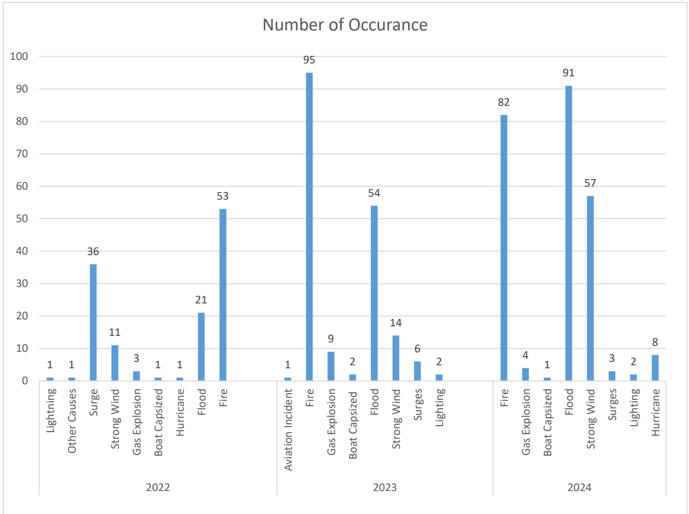
Figure 14: Types of hazards by year occurrences (Source; NDMA statistical report from 2021-2024)
